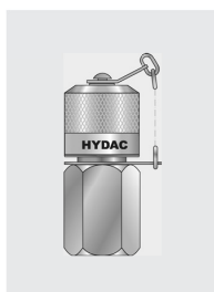
Standpipe adaptor 37° edged cone SAE J 514
